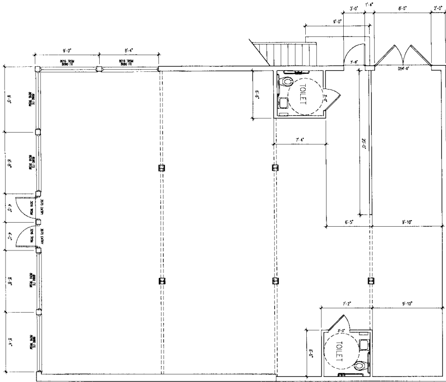
FIRST FLOOR SHOP PLAN SCALE: 1/8" = 1'-0"
