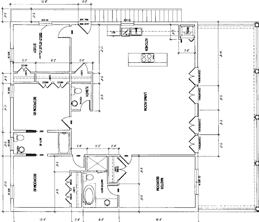
SECOND FLOOR RESIDENCE PLAN SCALE: 1/8" = 1'-0"
